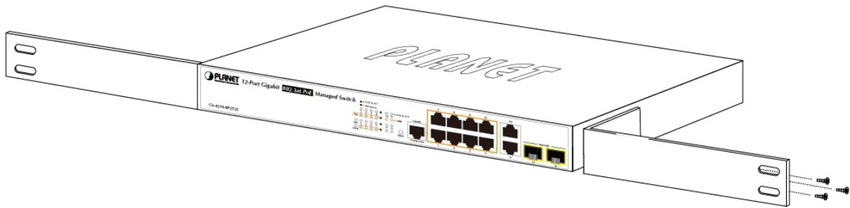
Figure 2-2-2: Attach Brackets to the Managed Switch.
