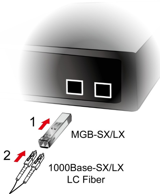
Figure 2-2-4: Plugging in the SFP/SFP+ Transceiver
